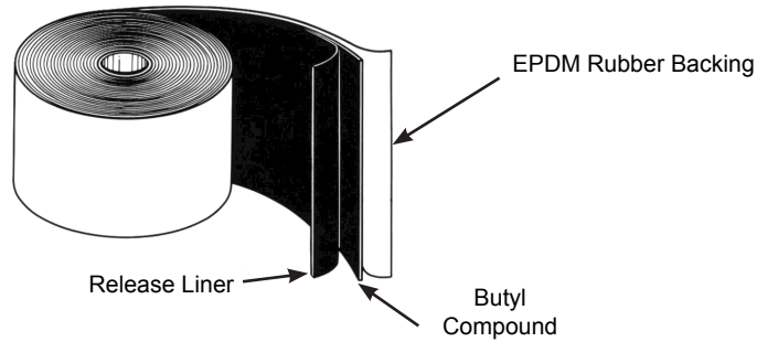
EZ-WRAP EPDM BACKED
